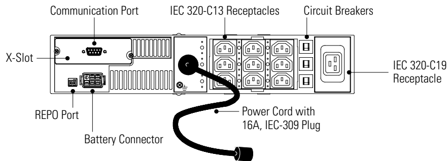
Figure 15. 2400–3000 VA, 230V Rear Panel
