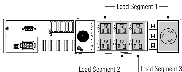
Figure 25. UPS Load Segments (120V Model Shown)
