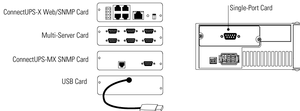
Figure 21. Optional X-Slot Cards
