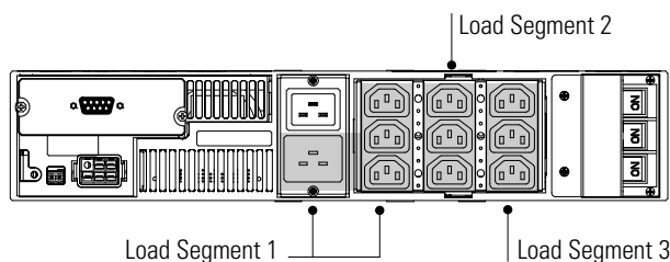
Figure 26. UPS Load Segments (PW5125 3000g RM Model Shown)
