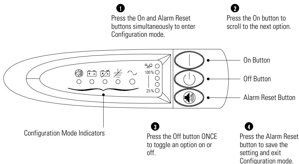
Figure 20. Using the Configuration Mode
